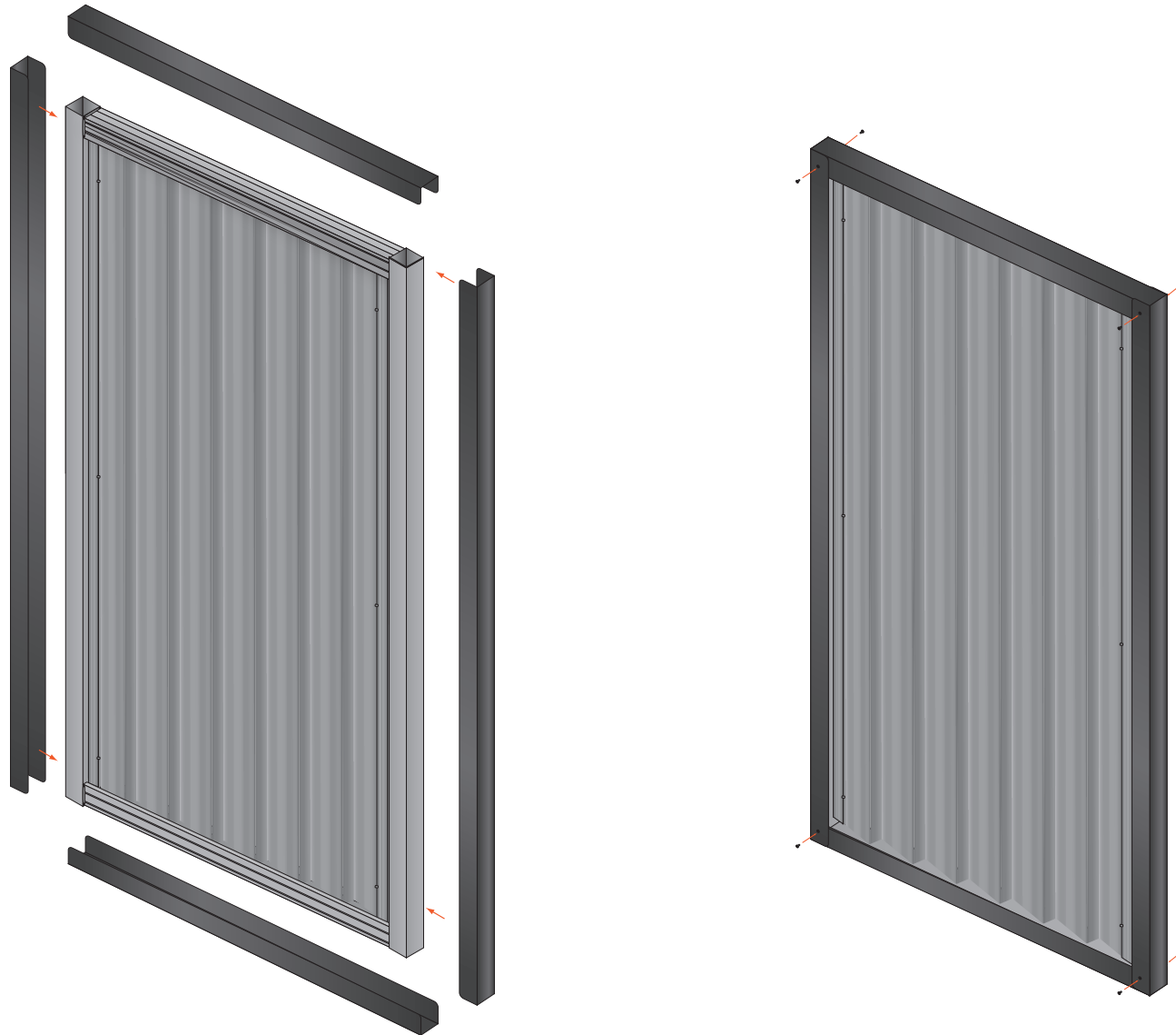
Powder coated ZINCANEAL® Steel Edge Capping pop rivetted to frame to create Dual Coloured Gate
