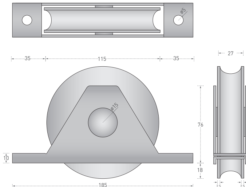
SLIDING GATE WHEEL
