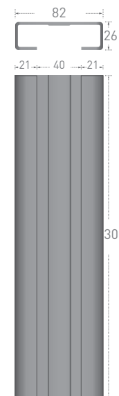
GUIDE CHANNEL
