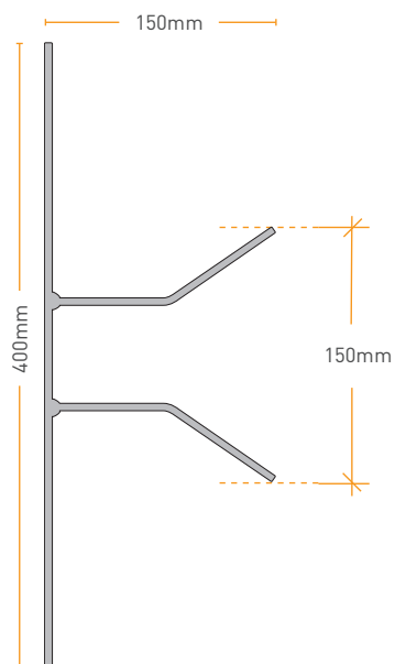
STANDARD F STOP
