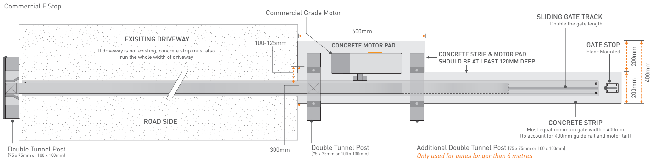
SLIDING GATE SETUP - TOP VIEW
